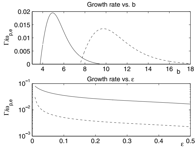
Figure 2. The normalized growth rate \Gamma/\omega_{p,e} for the distribution from equation (1) for a = 10 (solid line) and a = 20 (dashed line, exaggerated by a factor 5). The upper panel shows the growth rate for fixed \varepsilon = 0.4 . The lower panel shows the growth rate for fixed b = 5 (solid line) and b = 10 (dashed line). Note that the growth rate remains approximately constant as the asymmetry tends to, but is not precisely, zero.
