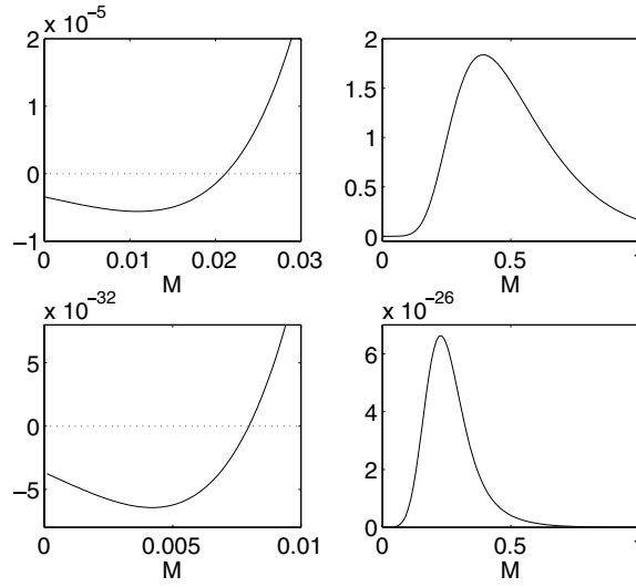
Figure 3. The function that determines the allowed (discrete) values for M , i.e., the left-hand side of equation (31) in T06b. Parameters are taken as a = 10 , b = 5 , and \varepsilon = 0.4 (upper panels) and \varepsilon = 0.499 (lower panels). For \varepsilon \rightarrow 0.5 (symmetric distribution), the function values become overall smaller (note the smaller scales in the lower panels) until, eventually, the function is equal to zero everywhere.
