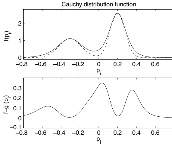
Figure 1. The counterstreaming Cauchy distribution function from equation (1) for the parameters a = 5 , b = 1 and \varepsilon = 0.3 (solid line) in comparison to a Maxwellian counterstreaming distribution function (dashed line) from equation (3). For larger values for a and b , the difference between the two distribution functions is negligible.
